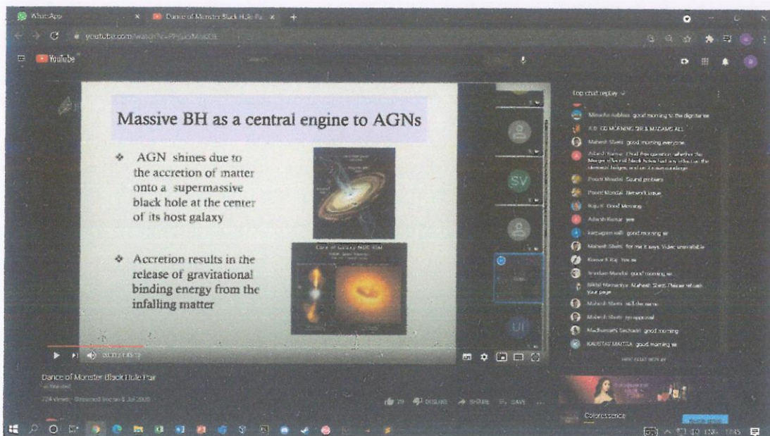
Monitoring the Cosmic Dance of the Monster Black Hole” ( 8 th July 2020 )
